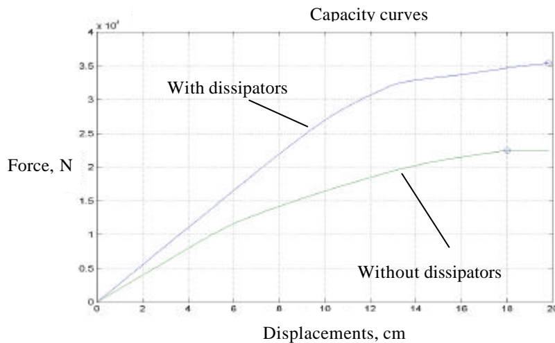
Figure 5: Capacity curves.
